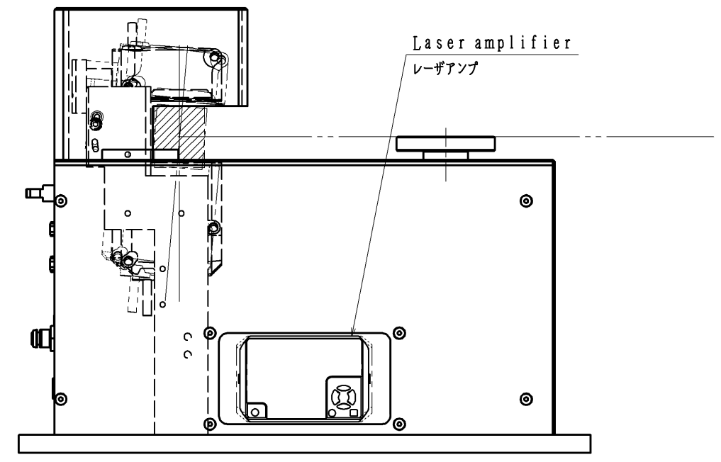
View A 矢視A
