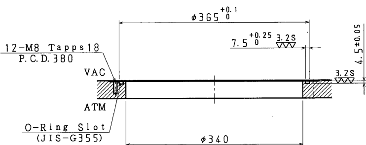
Chamber Attachment Seat Details (S=1:5)
